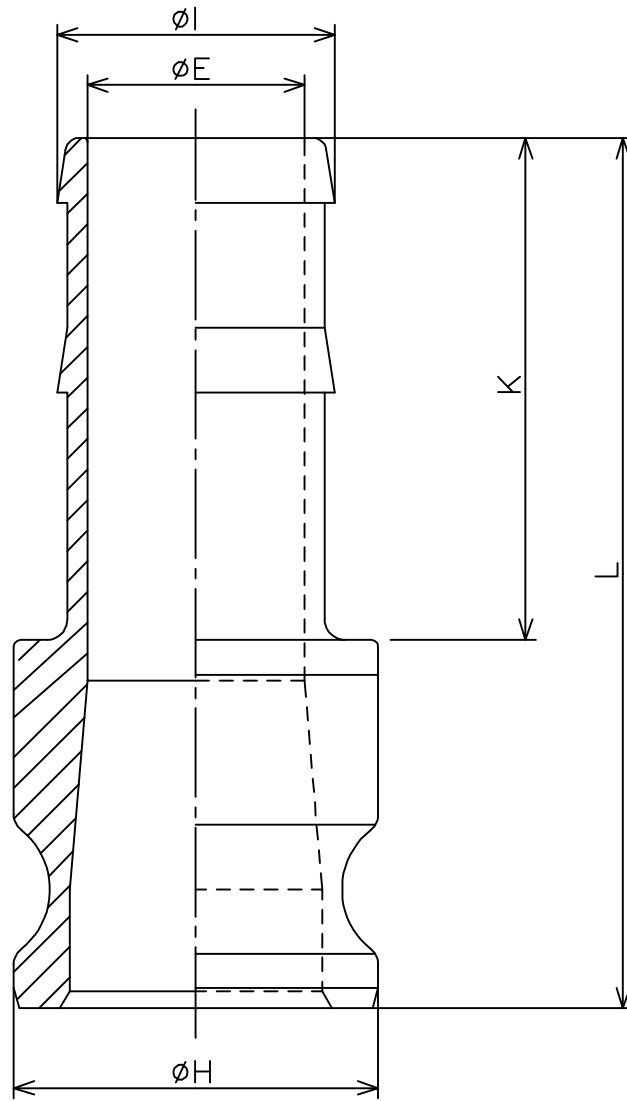
Dimensional sketch for Quick coupling -E
